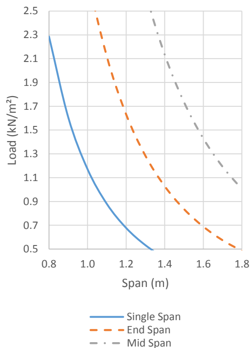
Load/Span
